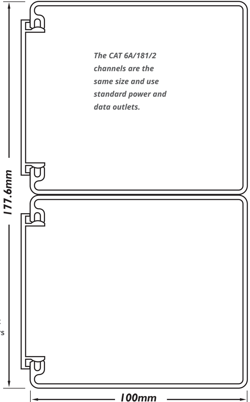
Covers - incl with Flat Bends 2 x 70.0470
