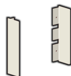
90 Degree End Cap Right and Left Ending. Rivet or screw fix to profiles. 150.2620
