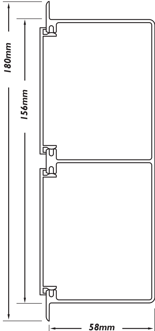
Joining Pieces Rivet or screw fix Supplied in pairs 156.2106
