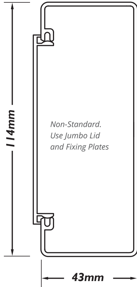
PDL 591CP Conversion Unit to allow standard power and data fittings (supply by others).
